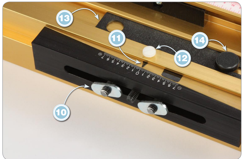
15 Sub Fence Mounting Hardware
