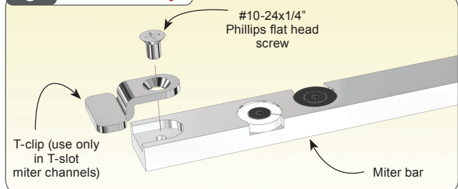
Fig. 3 Expand Miter Bar to Fit (front)
