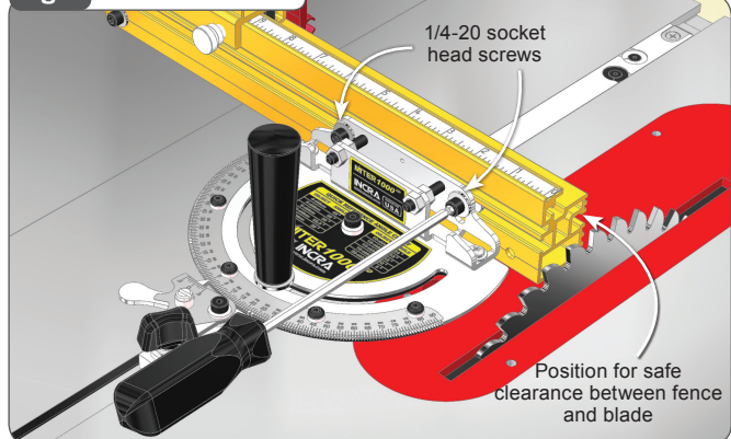
Fig. 5 Attach Fence
