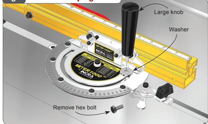
Fig. 2 Attach T-Clip
