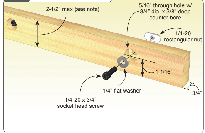
Fig. 18 Making a Sub Fence
